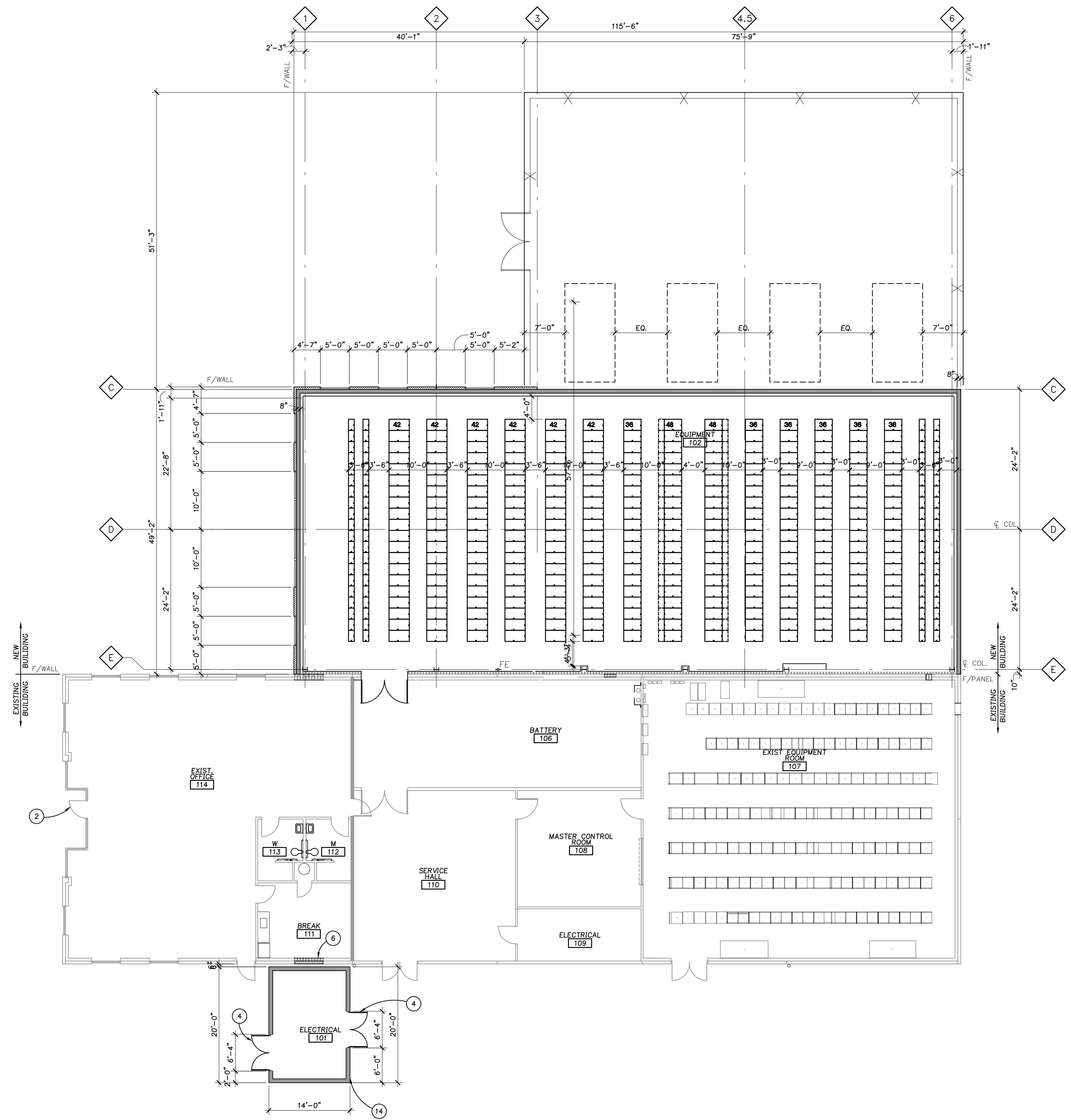
Floor Plan 1/8"=1'-0"
