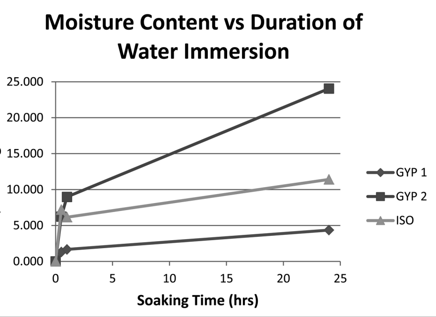
Figure 2 – Moisture content (% of original mass) vs. duration of water immersion (hours) for three cover board products. Each data point indicates an average of three or more samples.
