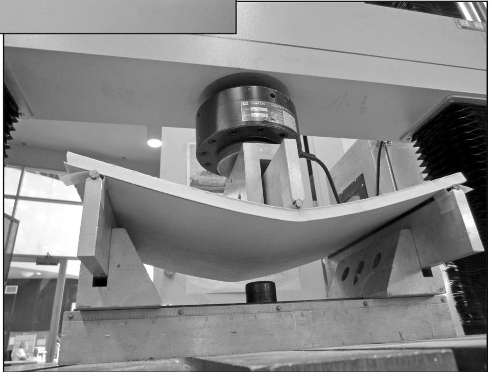
Photo 5 - Flexural test in progress.
