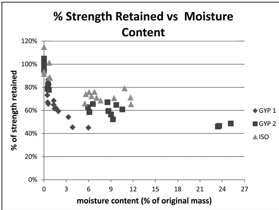
Figure 4 – Percent of original flexural strength retained vs. moisture content (% of original mass) for three cover board products. Each data point indicates one sample.
